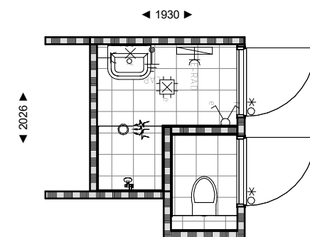
Basis opstelling
